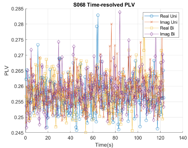
Time#Resolved PLV
