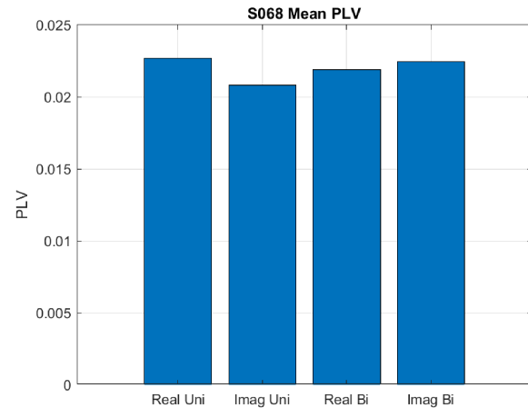
Mean PLV
