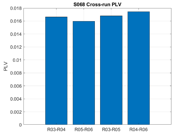
Cross#Run PLV
